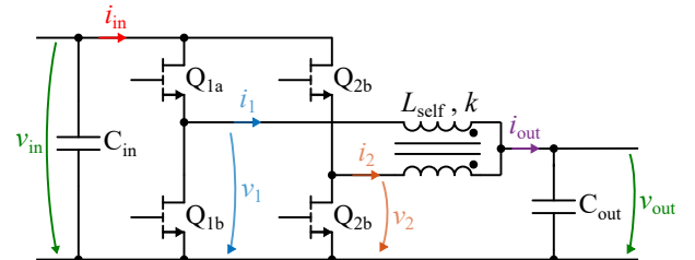
Fig. 1: Schematic of the Coupled Inductor Buck Converter.
